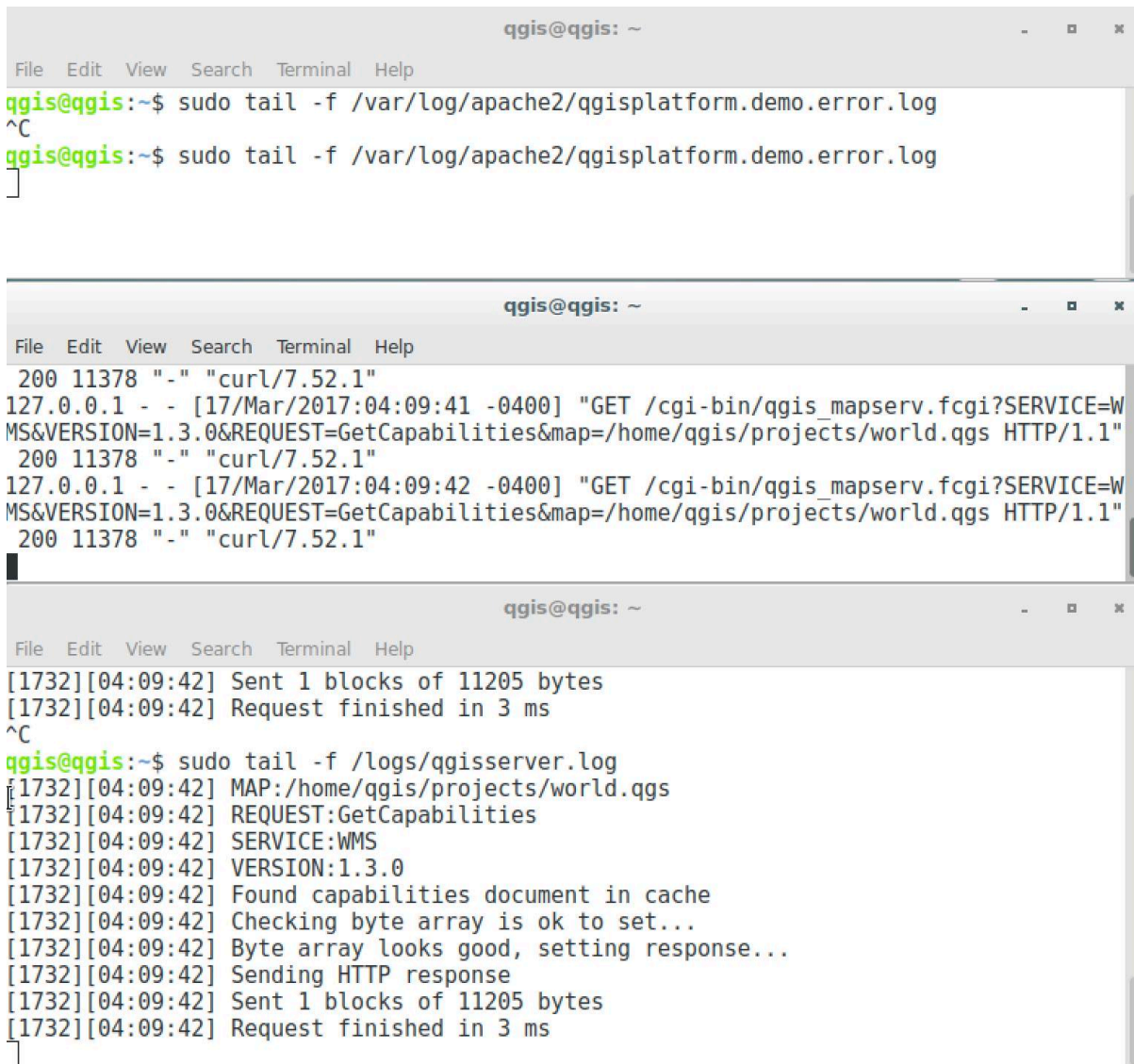
Şekil 11.2: Using the tail command to visualise QGIS Server logs output
