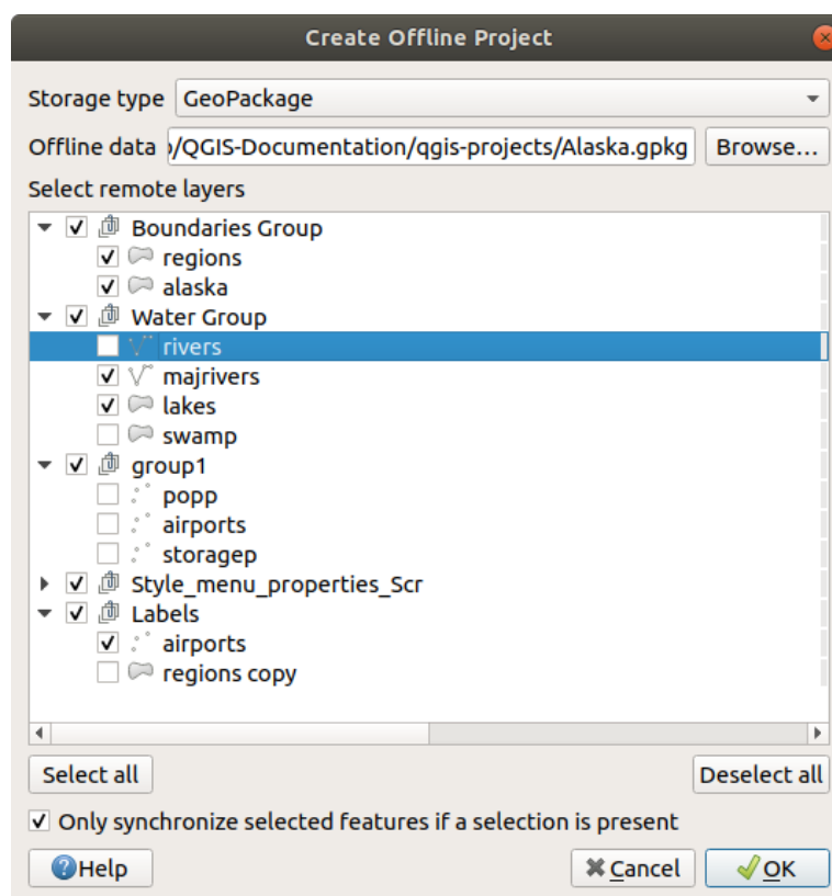
Рис. 24.27: Create an offline project
