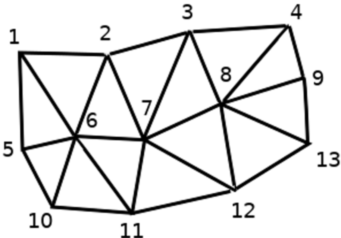
Рис. 16.2: Triangular grid with numbered vertices
