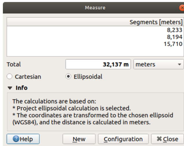
Рис. 11.17: Measure Distance
