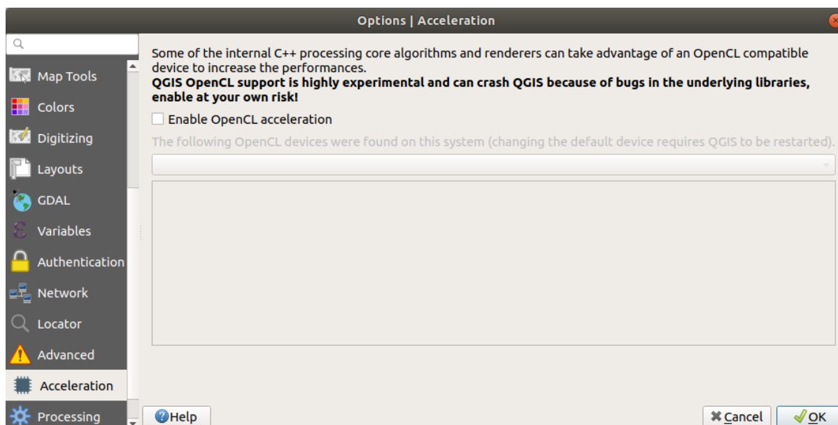
Рис. 9.18: Acceleration tab
