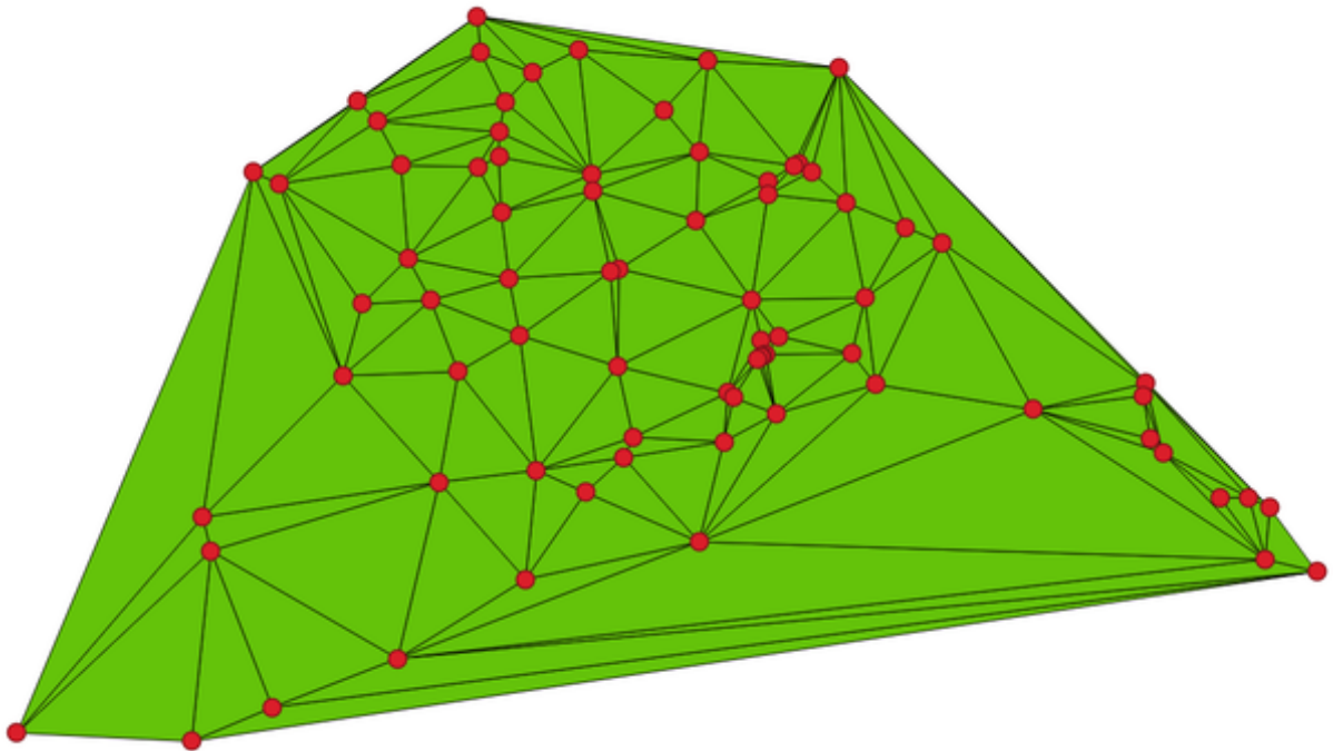
Рис. 23.38: Delaunay triangulation on points
