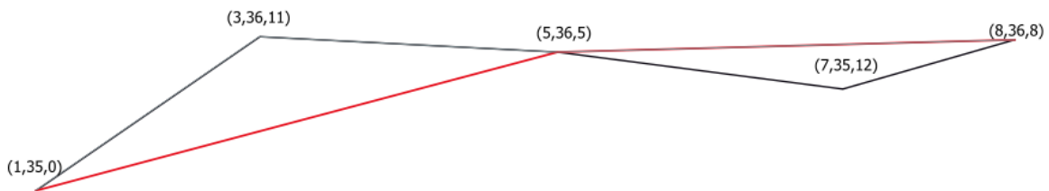
Рис. 23.47: The red line represents the black line with only vertices whose Z value is \leq 10 .
