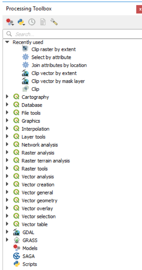
Рис. 22.6: Processing Toolbox
