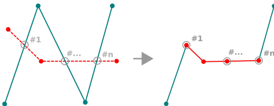
Рис. 14.91: Reshape line
