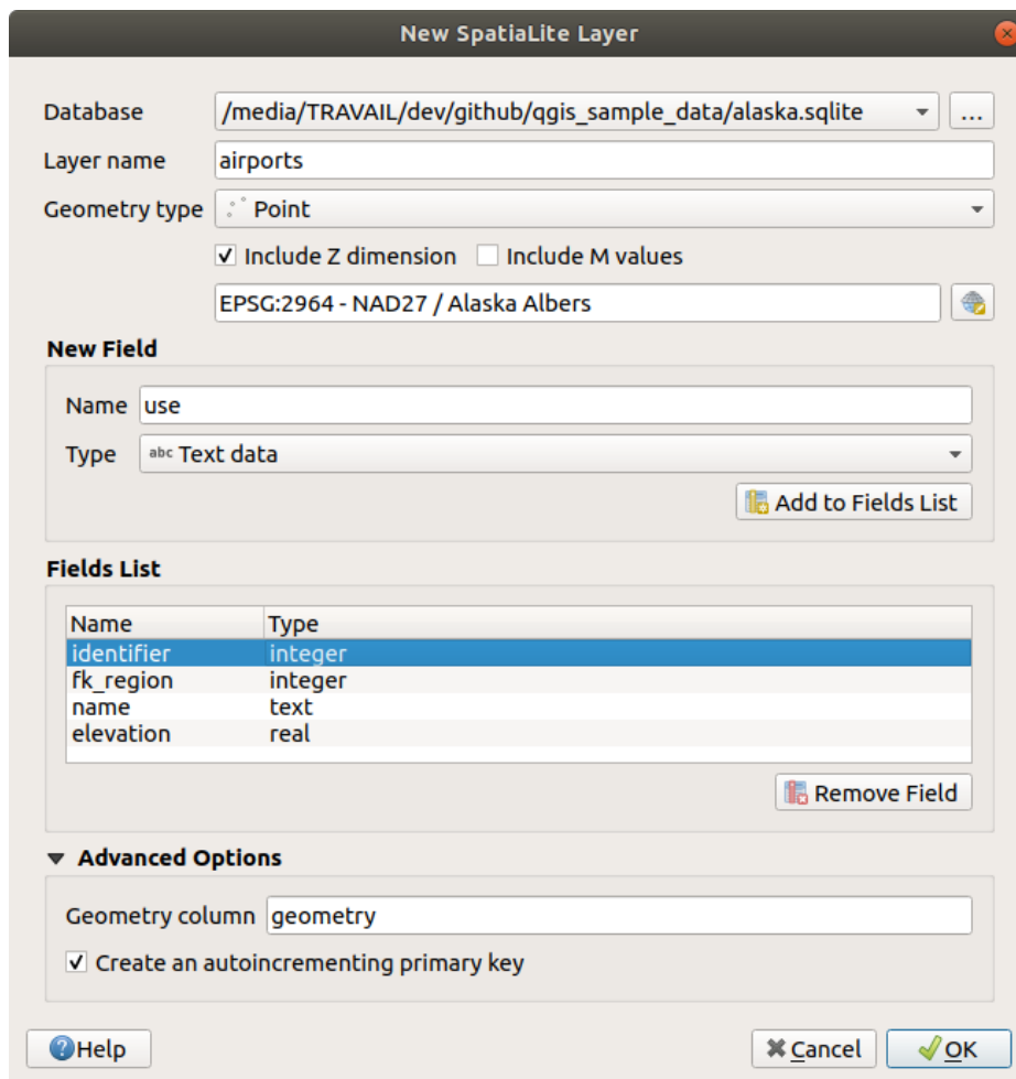
Рис. 13.15: Creating a New SpatiaLite layer dialog
