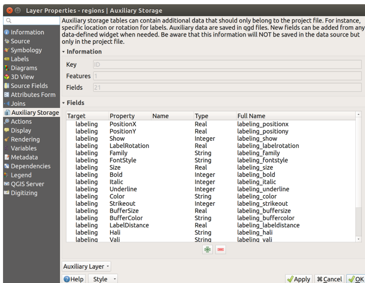
Рис. 14.49: Auxiliary Fields
