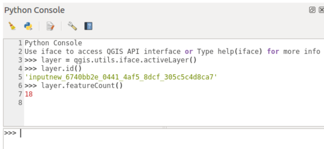
Fig. 1.1: QGIS Python-console
