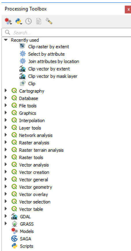
Fig. 22.1: Processing Toolbox
