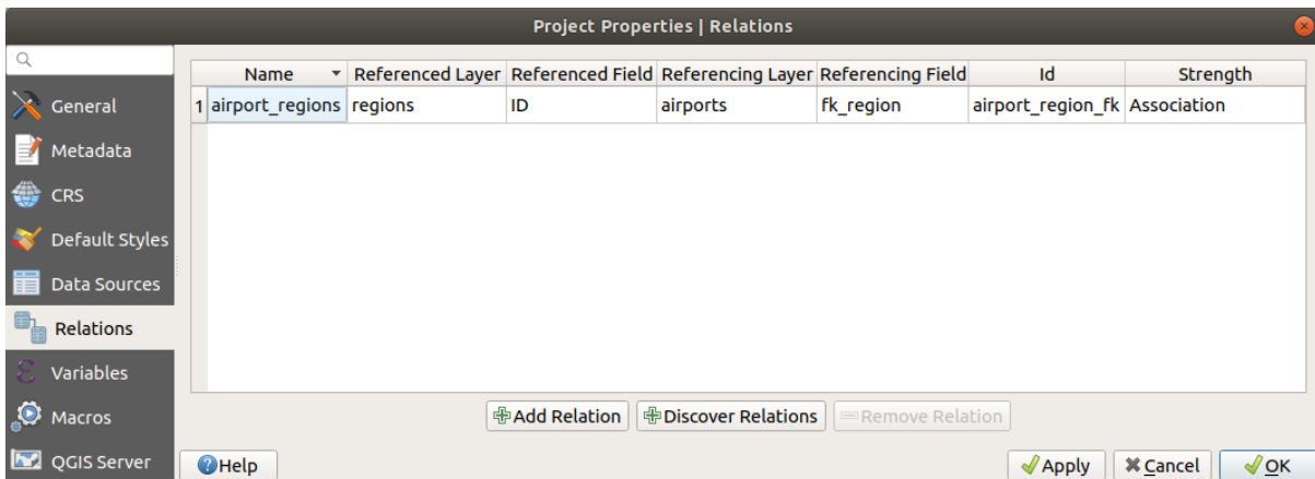
Fig. 9.23: Relations tab
