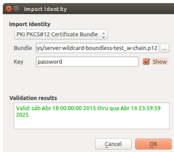
Obr. 20.31: PKCS#12 identity import
