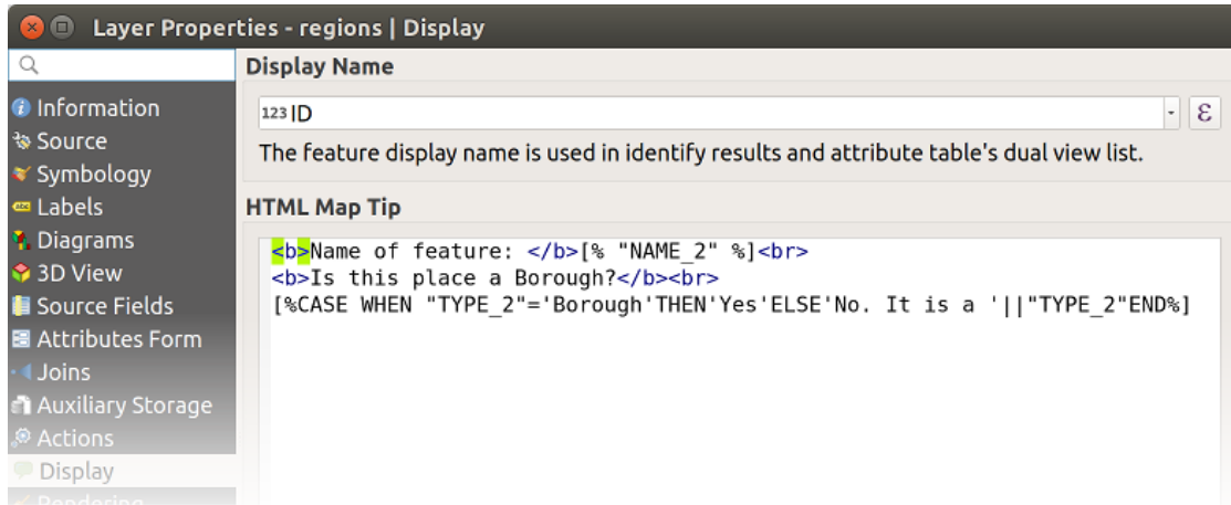
Obr. 14.59: HTML code for map tip
