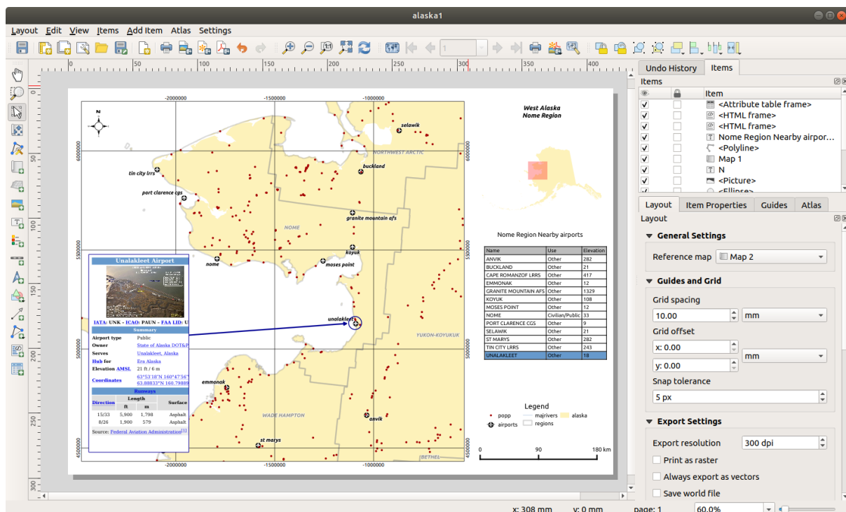
Obr. 17.56: Print Layout with map view, legend, image, scale bar, coordinates, text and HTML frame added
