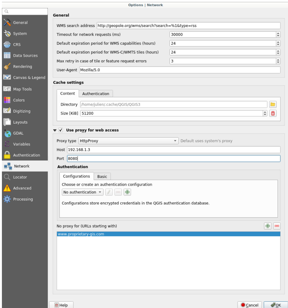
Obr. 9.15: Proxy-settings in QGIS
