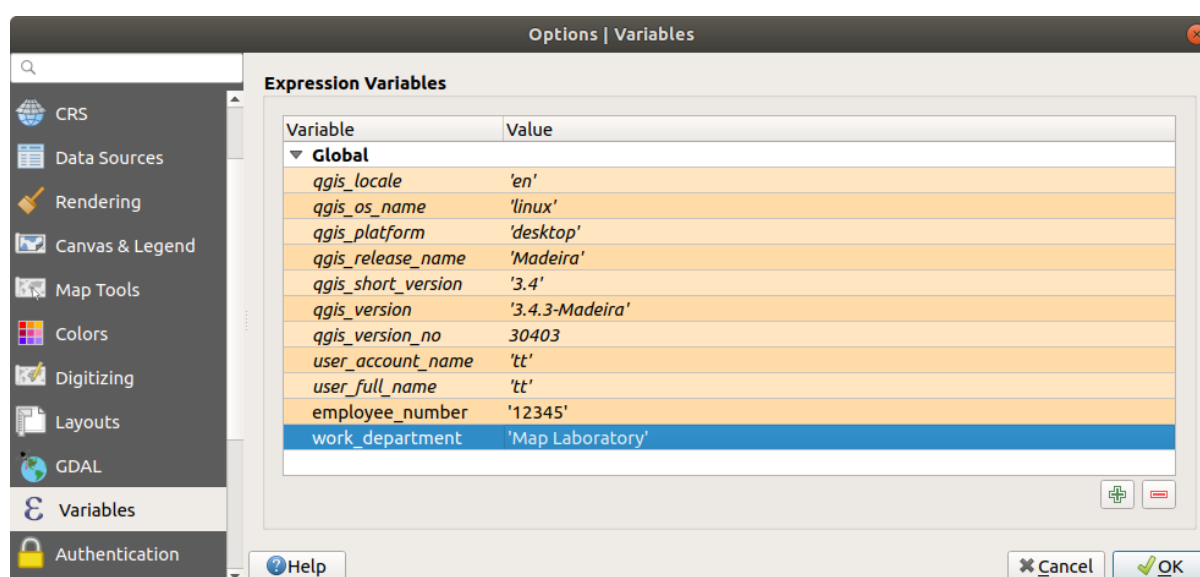
Obr. 9.13: Variables Settings in QGIS
