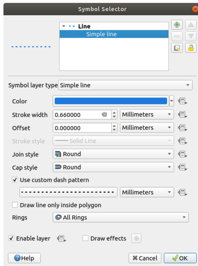
Obr. 12.10: Designing a Simple Line Symbol
