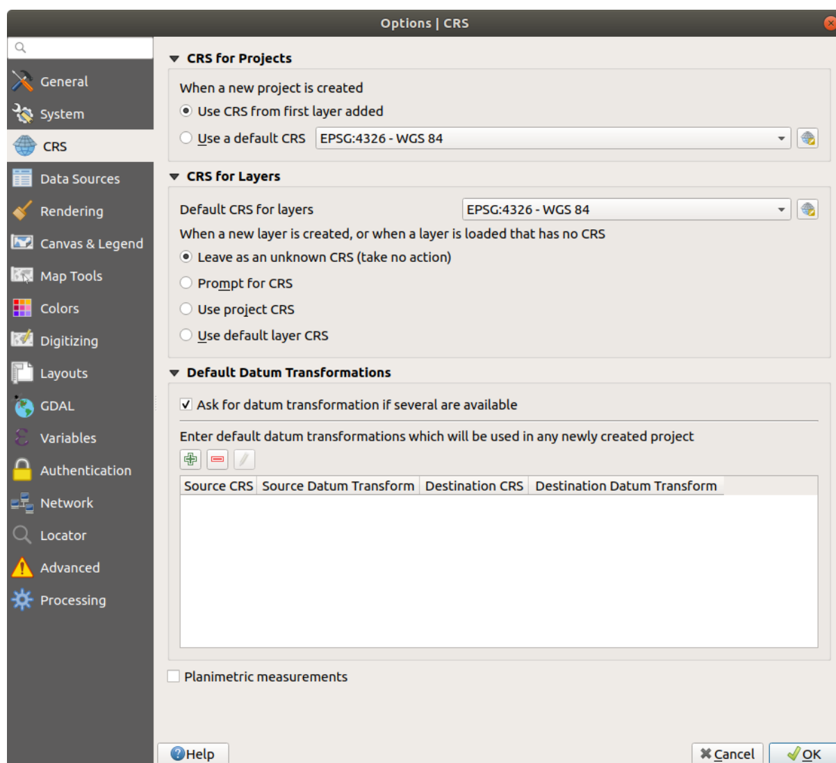
Obr. 10.1: The CRS tab in the QGIS Options Dialog
