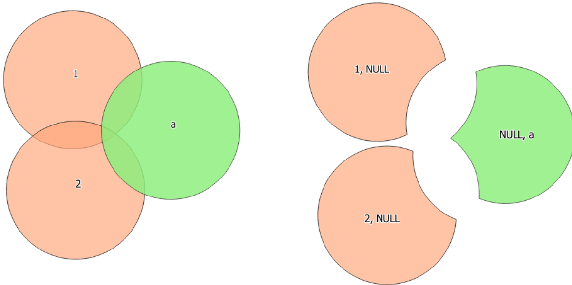
Obr. 23.83: Symmetrical difference operation between a two-features input layer and a single feature overlay layer (left) - resulting features are moved for clarity (right)
