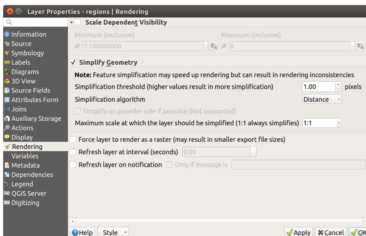
Obr. 14.61: Layer Geometry Simplification dialog
