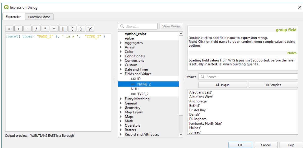
Obr. 14.65: The Expression tab
