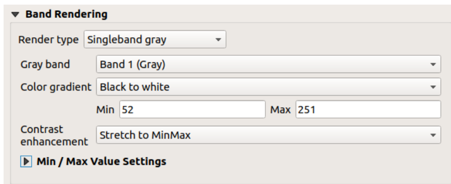
Obr. 15.4: Raster Symbology - Singleband gray rendering
