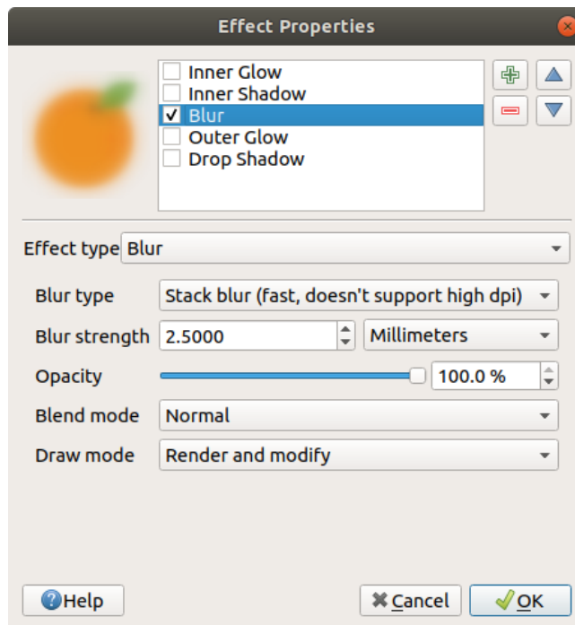
Obr. 14.19: Draw Effects: Blur dialog
