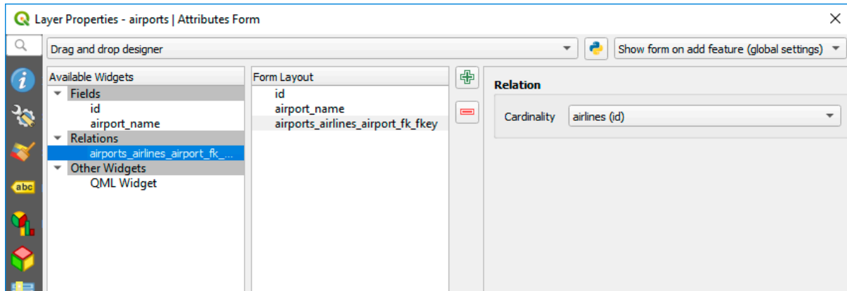
Obr. 14.82: Set relationship cardinality
