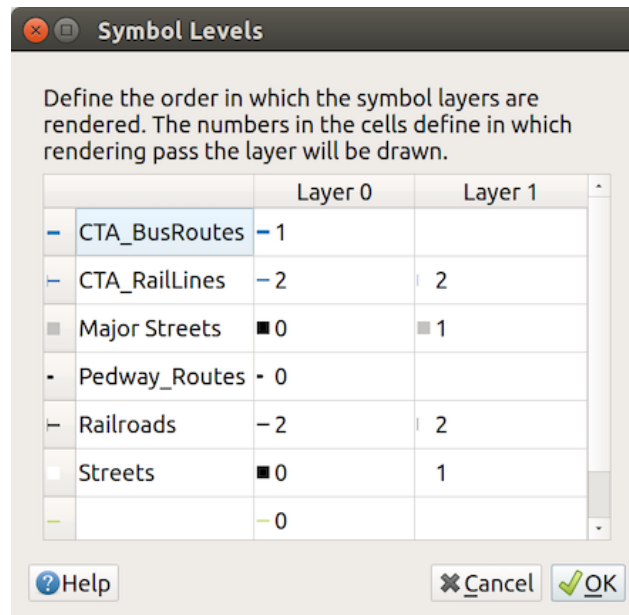
Obr. 14.15: Symbol levels dialog
