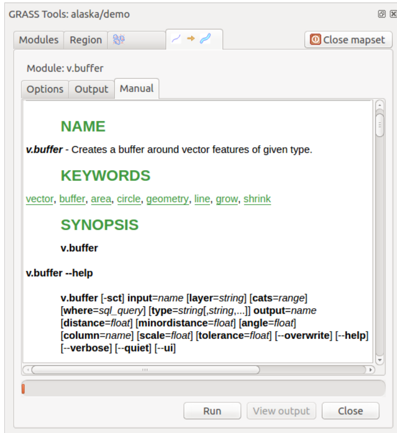
Obr. 21.6: GRASS Toolbox Module Manual
