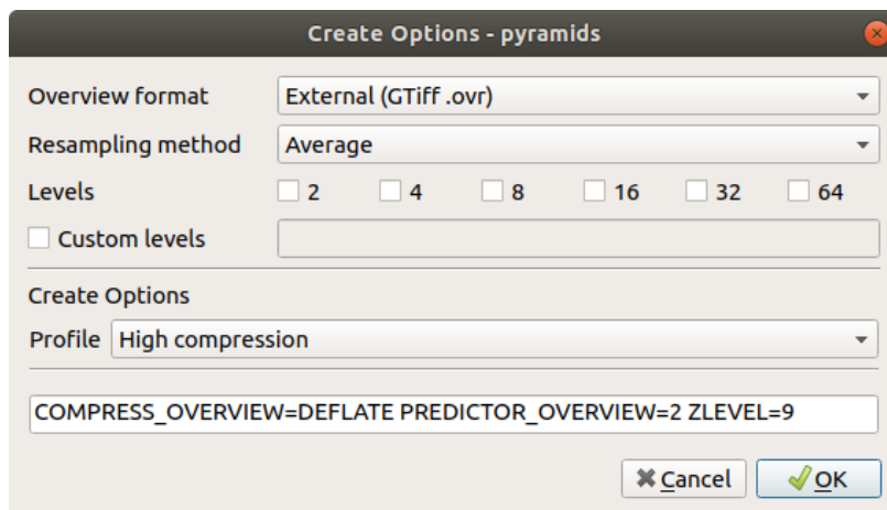
Obr. 9.11: Sample of Pyramids profile
