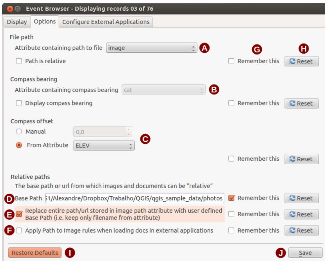
Obr. 24.12: The eVis Options window
