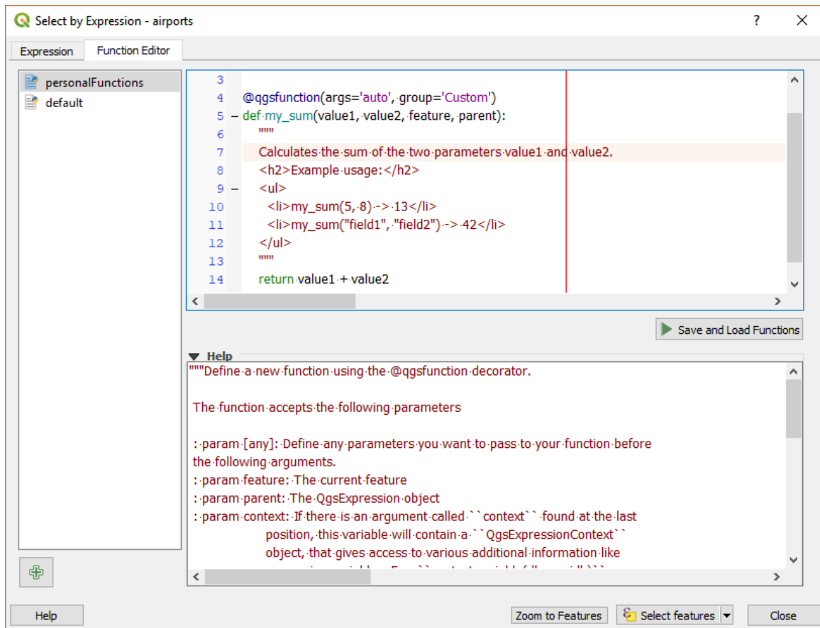
Obr. 14.66: The Function Editor tab
