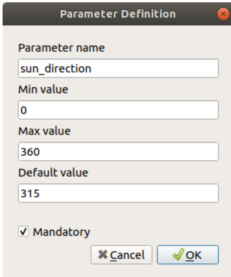
Obr. 22.19: Model Parameters Definition
