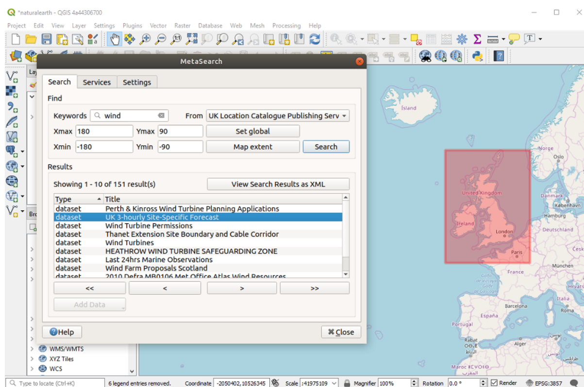
Fig. 24.22: Search and results of Services in MetaSearch
