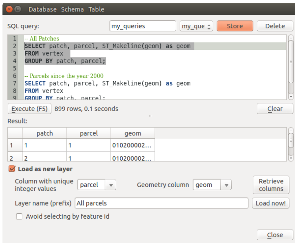
Рис. 19.8: Executing SQL queries in the DB Manager SQL window 🐧
