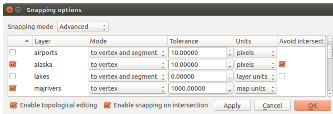
Рис. 12.40: Edit snapping options on a layer basis (Advanced mode) 🐧
