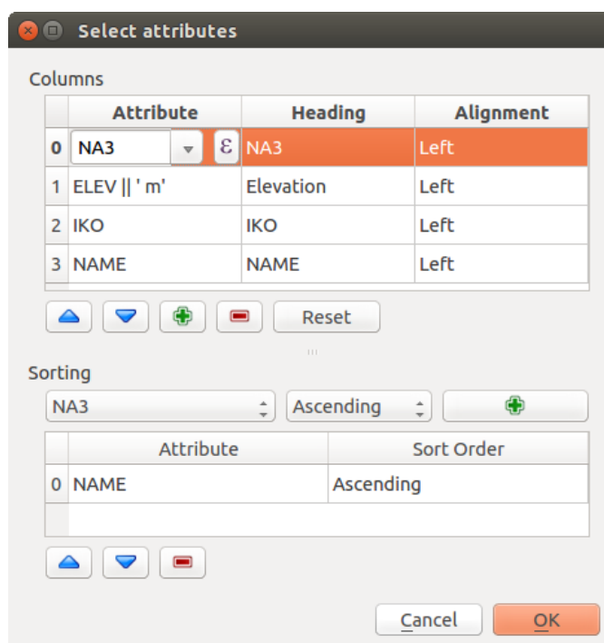
Рис. 18.30: Attribute table Select attributes Dialog 🐧
