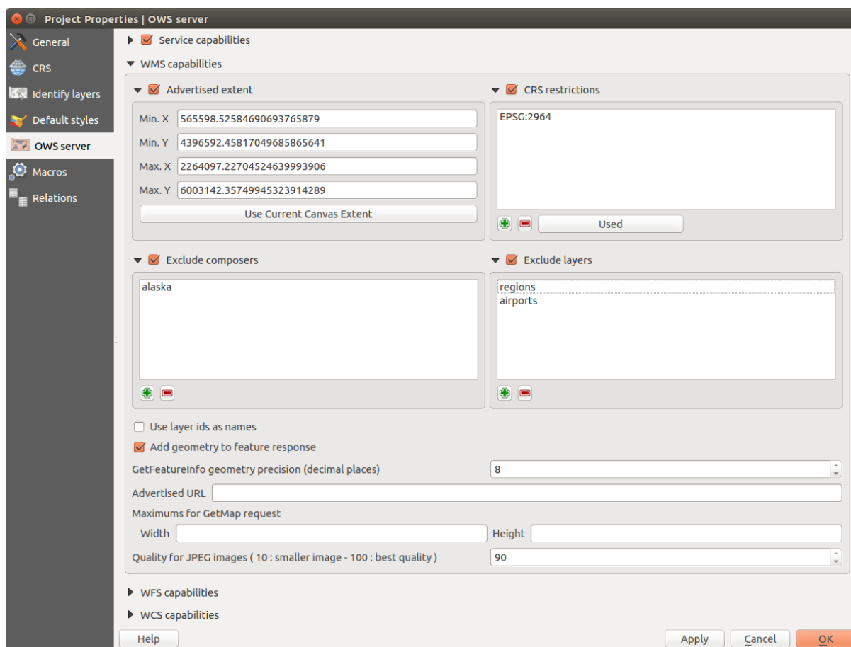
Рис. 14.5: Definitions for a QGIS Server WMS/WFS/WCS project (KDE)
