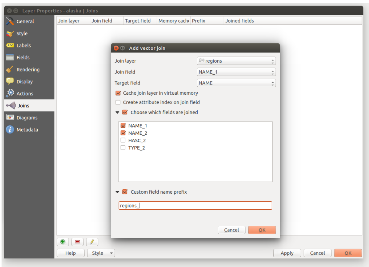
Рис. 12.36: Join an attribute table to an existing vector layer 🐧
