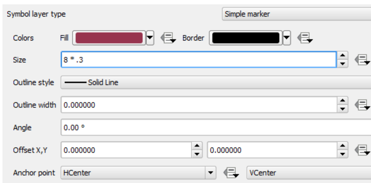
Рис. 12.12: Expression in Size spinbox 🐧
