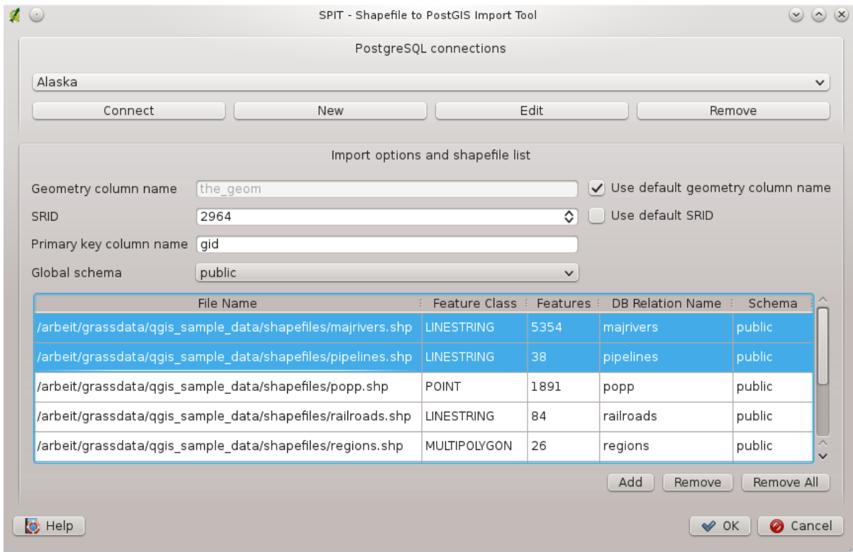
Figure 19.31: Using SPIT Plugin to import Shape files to PostGIS 🐧
