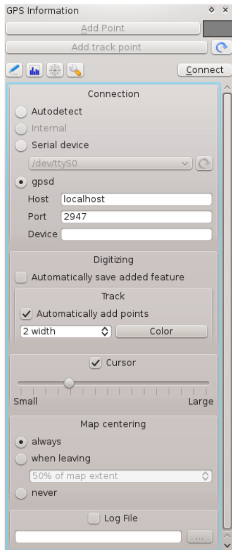
Figure 15.6: GPS tracking options window 🐧
