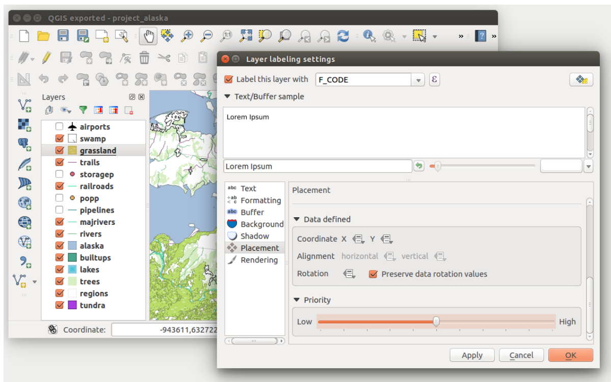
Рис. 12.39: Labeling of vector polygon layers with data-defined override
