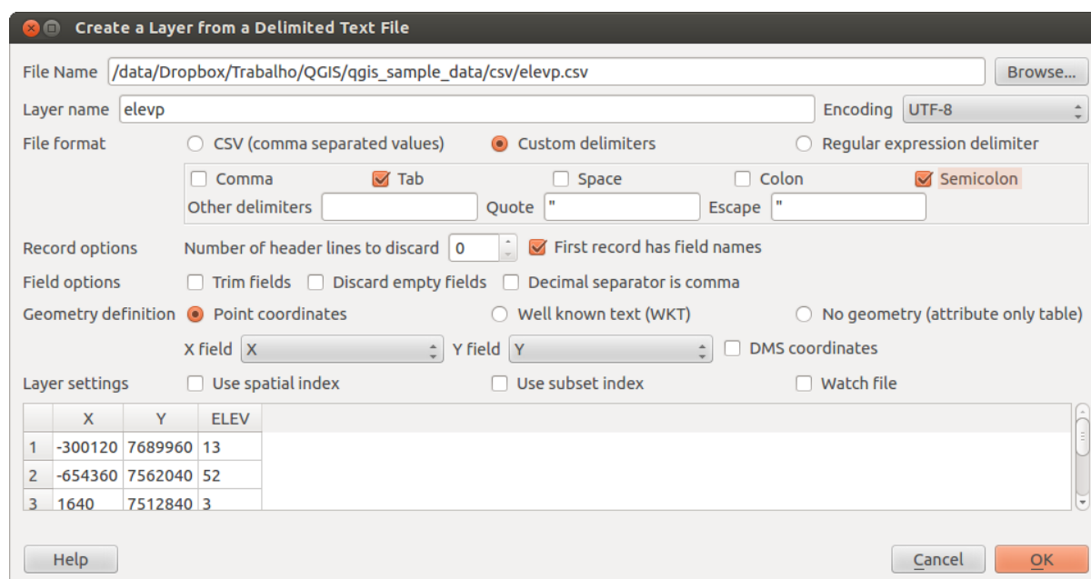
Рис. 12.4: Delimited Text Dialog
