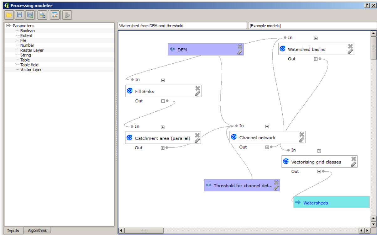
Рис. 18.2: Processing Modeler
