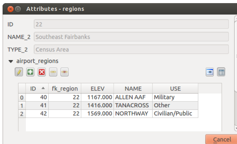
Рис. 12.65: Identification dialog regions with relation to airports
