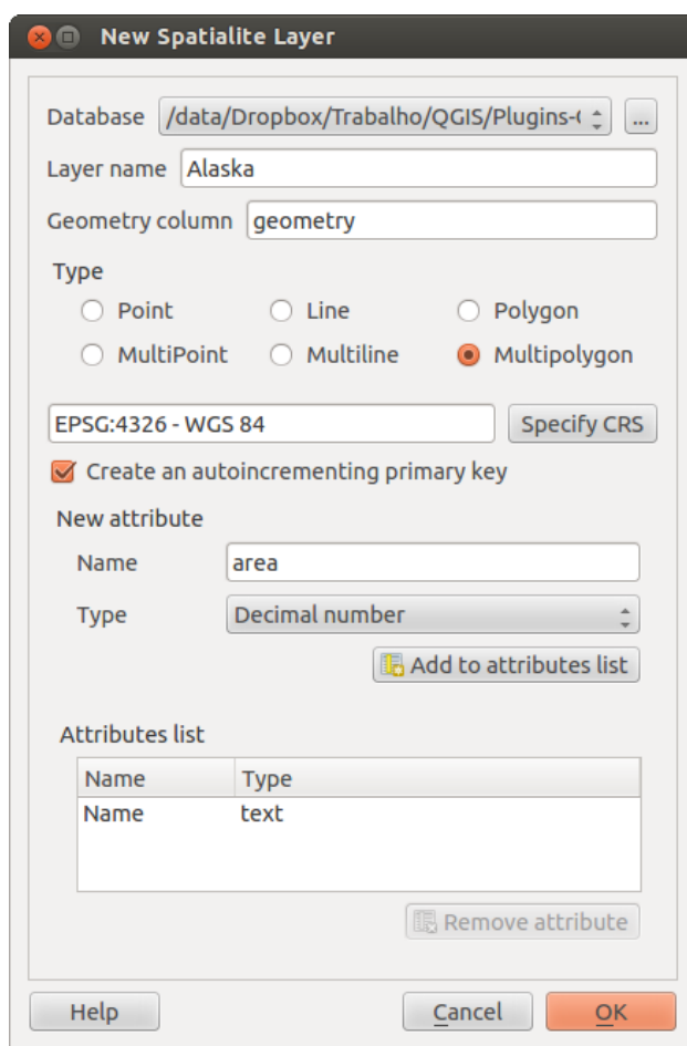
Рис. 12.74: Creating a New Spatialite layer Dialog
