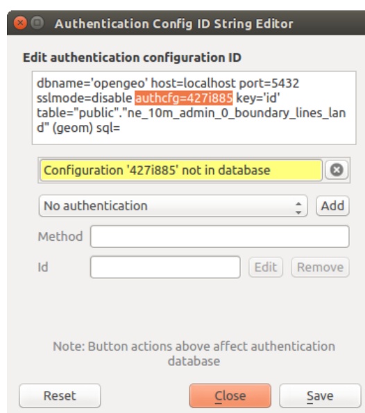
Рис. 16.31: Edit bad layer's authentication config ID
