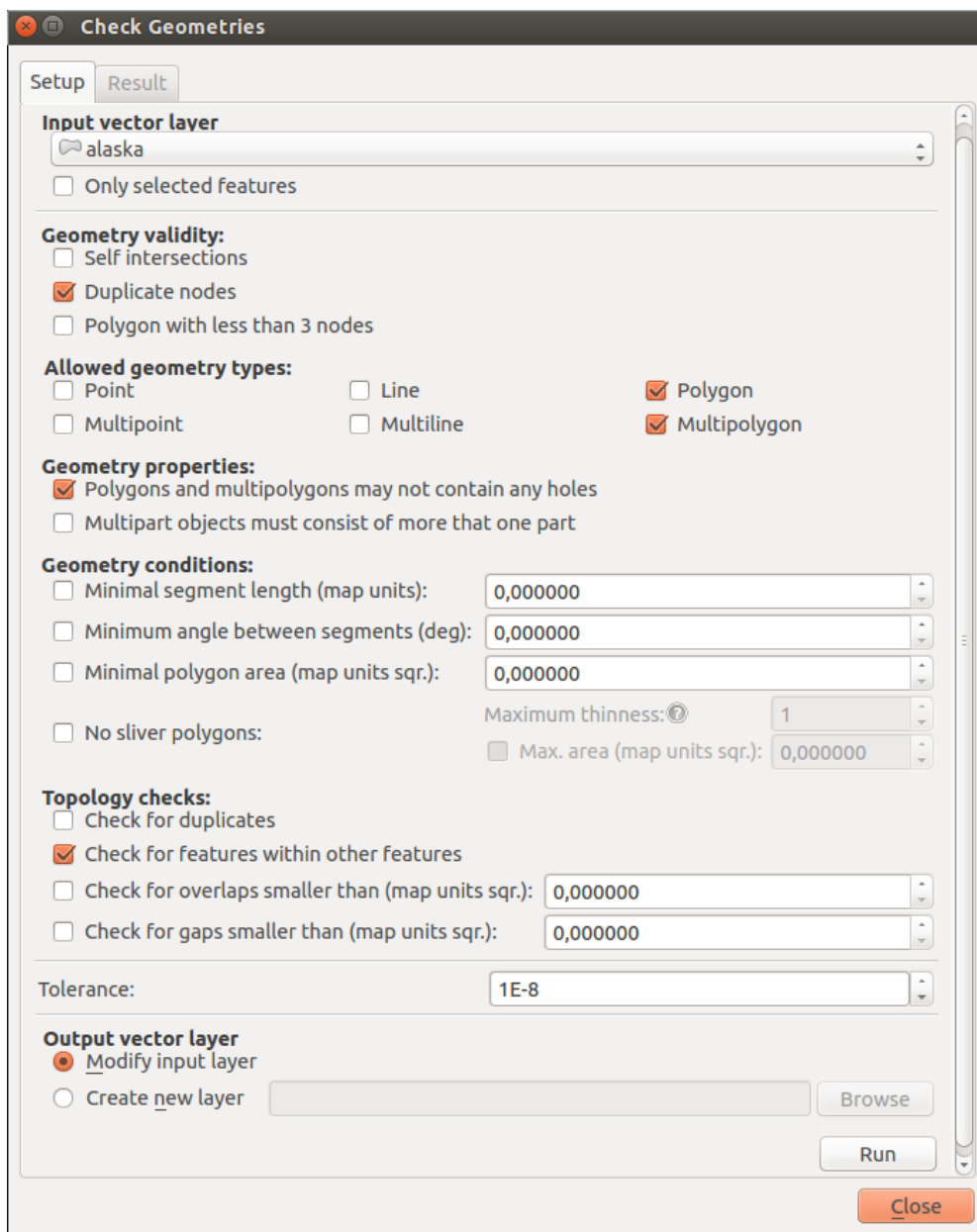
Рис. 20.17: The Geometry Checker Plugin
