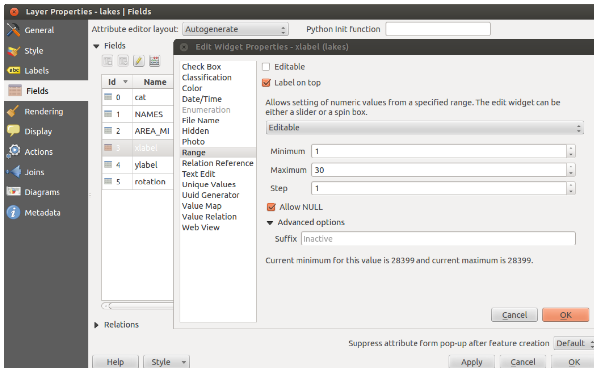
Рис. 12.43: Dialog to select an edit widget for an attribute column
