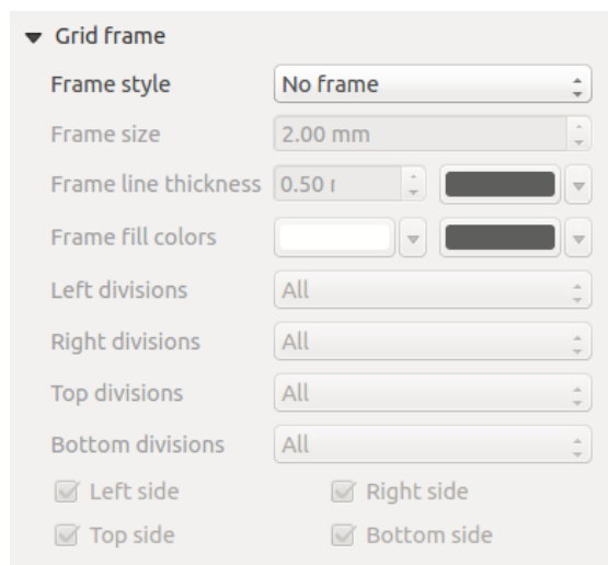
Рис. 19.14: Grid Frame Dialog
