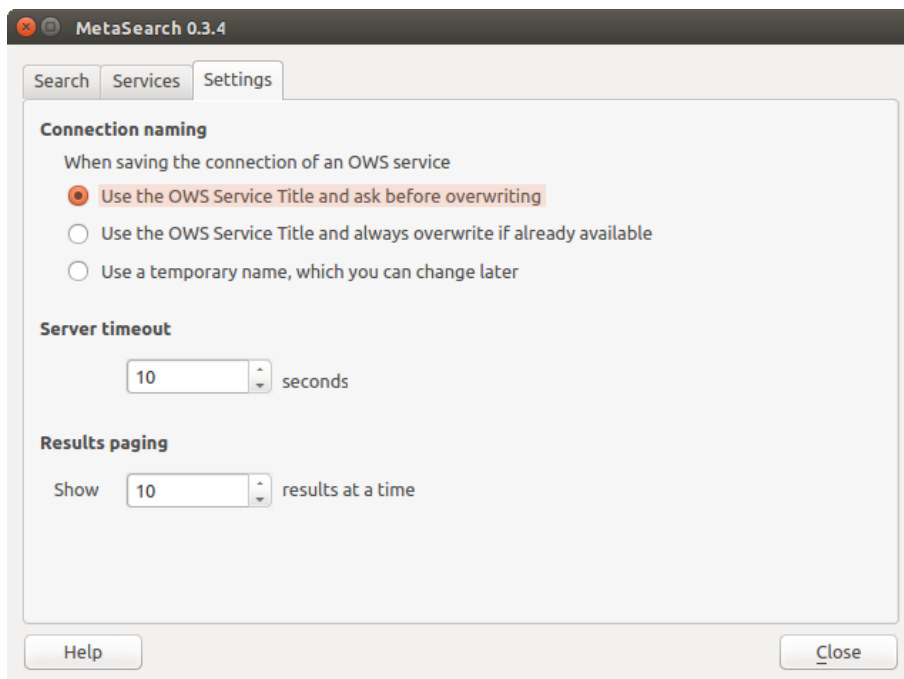
Рис. 20.31: Metasearch setting
