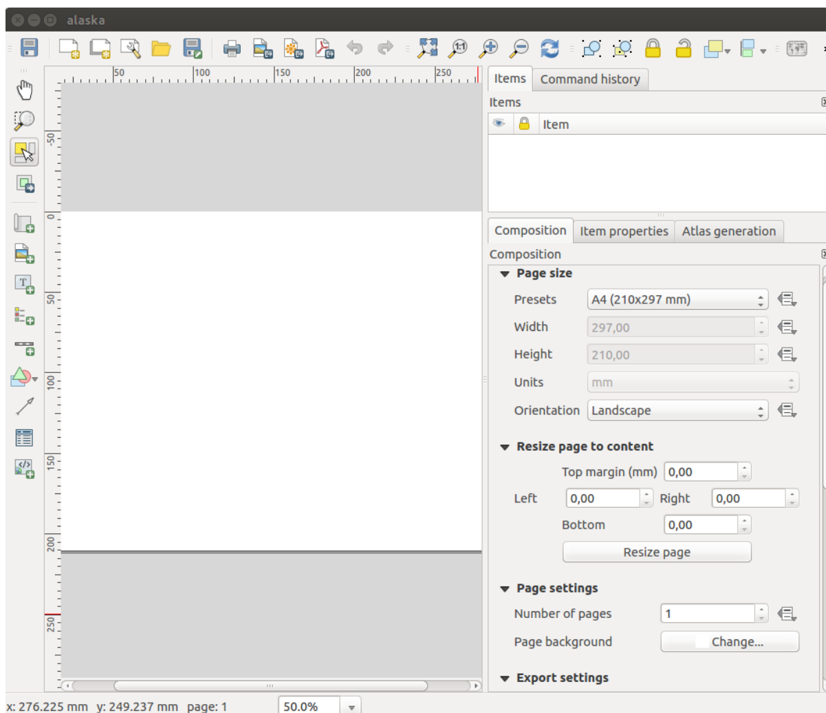
Рис. 19.2: Print Composer
