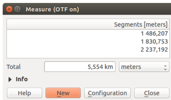
Рис. 8.5: Measure Distance
