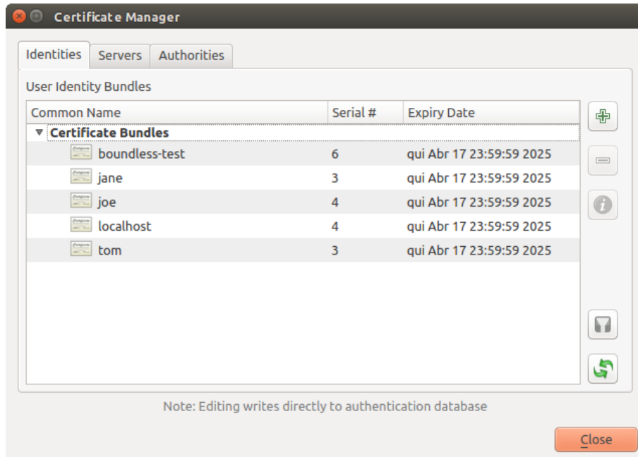
Figure 16.27: Identities editor
