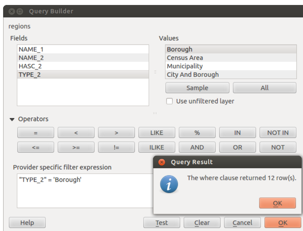
Figure 12.14: Query Builder
