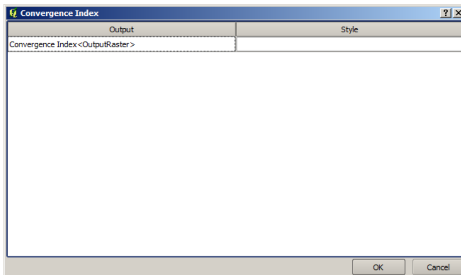
Figure 18.16: Rendering Styles
