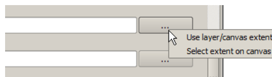
Figure 18.11: Extent selector
