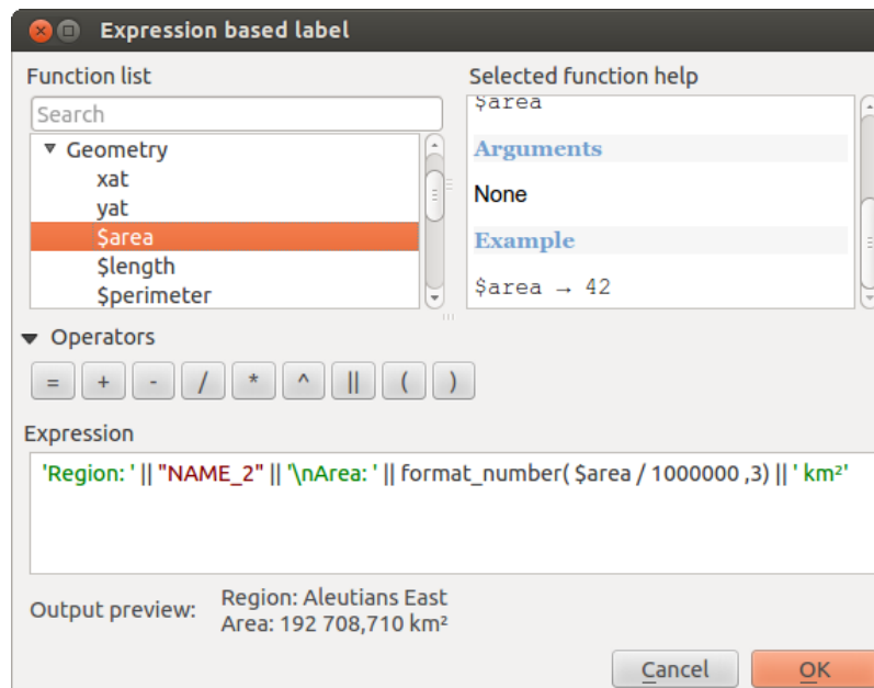
Figure 12.38: Using expressions for labeling
