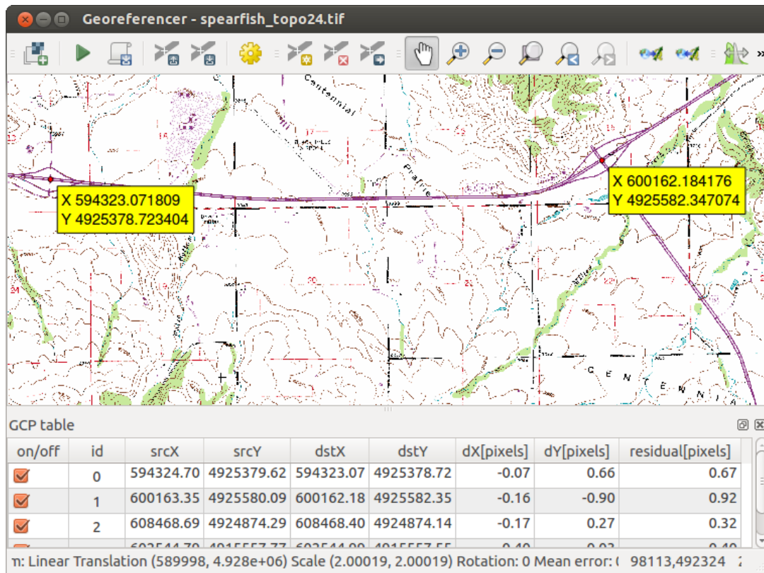
Рис. 19.17: Georeferencer Plugin Dialog
