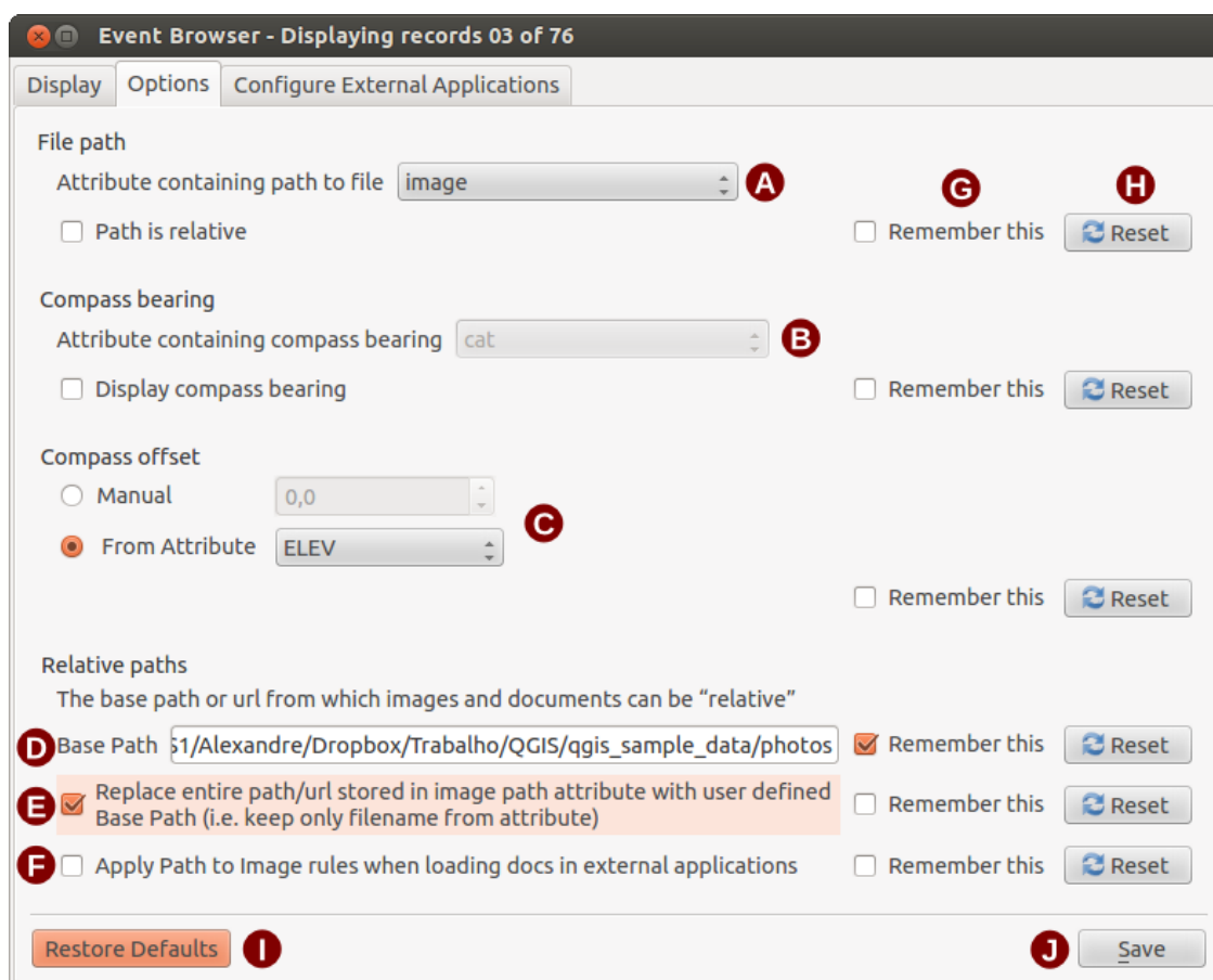
Рис. 19.11: The eVis Options window
