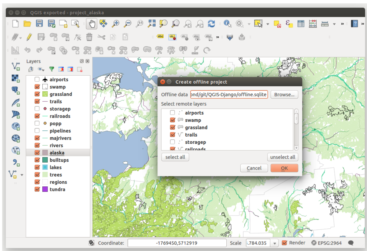
Рис. 19.25: Create an offline project from PostGIS or WFS layers
