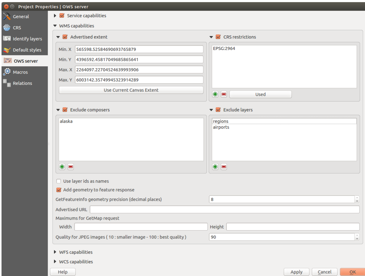
Рис. 14.5: Definitions for a QGIS Server WMS/WFS/WCS project (KDE)
