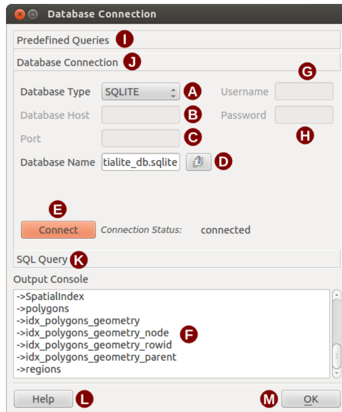
Fig. 19.13: The eVis Database connection window
